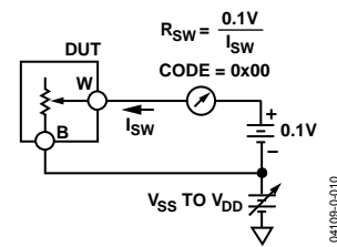
Figure 34. Test Circuit for Incremental On Resistance
